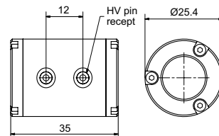
Outline drawing of D-compact/9
