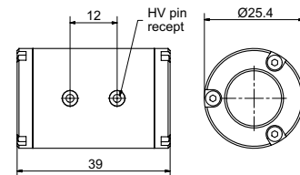
Outline drawing of D-compact/12
